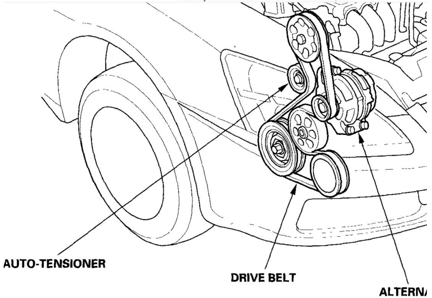
Fig. 1: Identifying Components Of Charging System Courtesy of AMERICAN HONDA MOTOR CO., INC.
